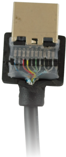
Standard 940 Series Over Mold and Construction
